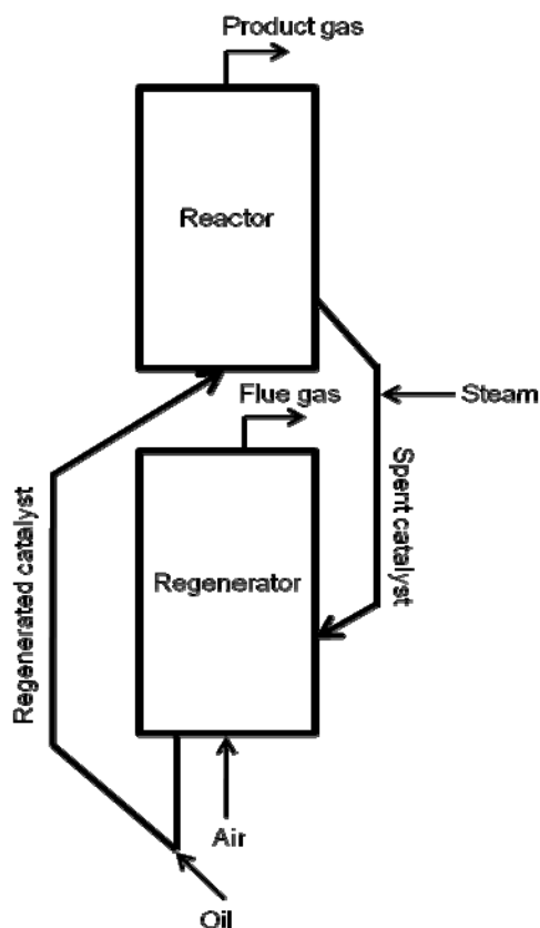
Figure 4 Schematic picture of an FCC-unit[15]
