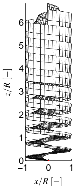
Figure 4.32: Vortex lattice prescribed wake. Wake geometry for one blade in the x-z plane normalized by the blade radius
