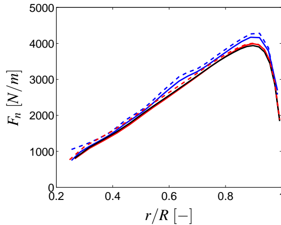
Figure 4.61: Distribution of the normal force along the blade, —: LLPW , —: VLPW , —: VLFW , - - - : BEM , - - - : GENUVP
