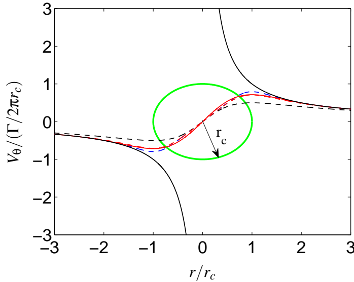
Figure 2.3: Tangential velocity of ideal vortex, Lamb-Oseen model and Vasisas model, —: Ideal vortex, —: Lamb-Oseen, - - - - : n = 1 , - . - . : n = 2 , - - - - : n = 3 , —: Vortex core
