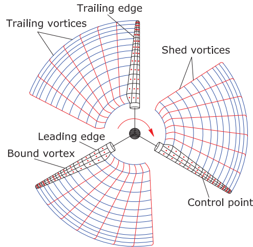
Figure 3.17: Schematic of vortex lattice free wake
