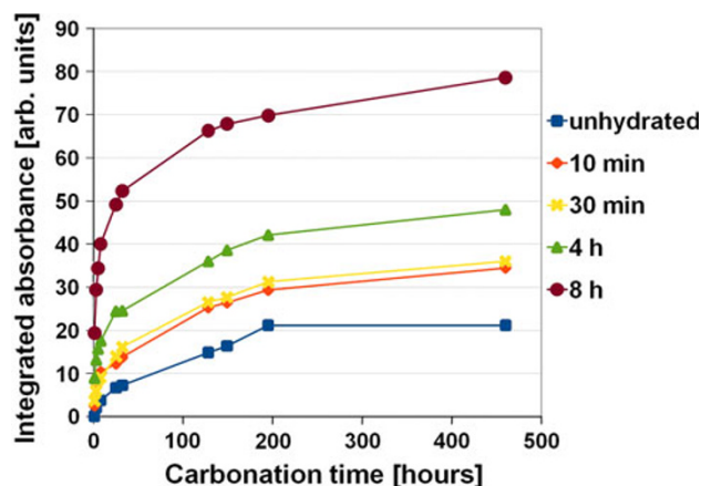
Fig. 3 Integrated peak areas for unhydrated and hydrated samples exposed to ambient air as a function of exposure time. The integration range was 1,300\text{--}1,700\text{ cm}^{-1} (marked as dotted lines in Fig. 2), where the zero-level was set at 1,300\text{ cm}^{-1} . The sample exposed for 10 min was used as reference for each hydration time.
