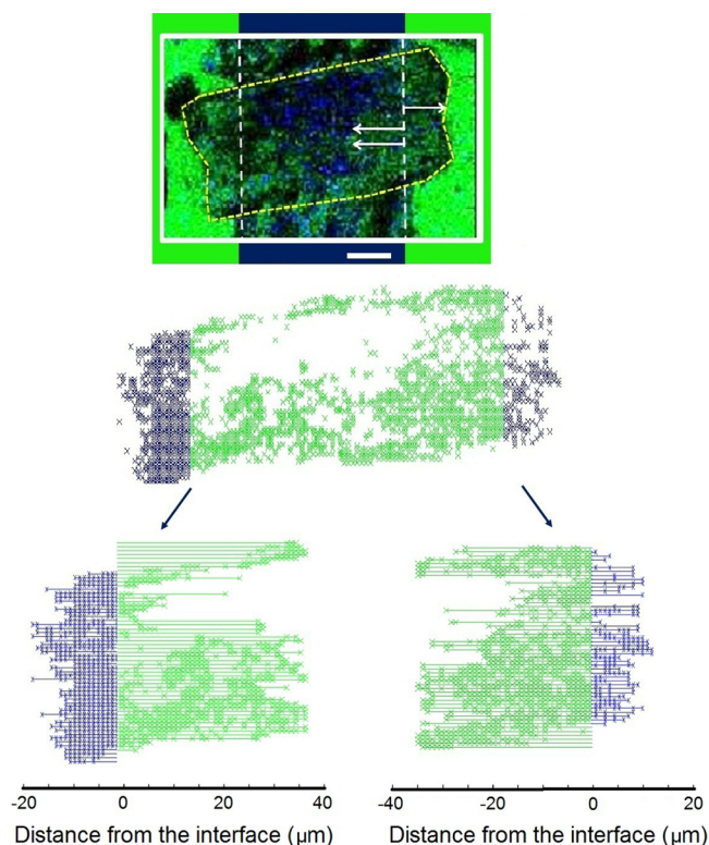
Figure 6. Migration distance of PEG and lipid molecules in a single matrix crystal was measured using TOF-SIMS imaging and the device. TOF-SIMS image of a single matrix crystal is isolated (top); pixels in the PEG region that contained lipid peaks with S/N > 3 (middle, green) and pixels in the lipid region of the device that contained lipid peaks with S/N > 3 (middle, blue) are isolated, and the distance between these pixels and the PEG-lipid interface is measured (bottom). The scale bar shows 20 \mu\text{m} .
