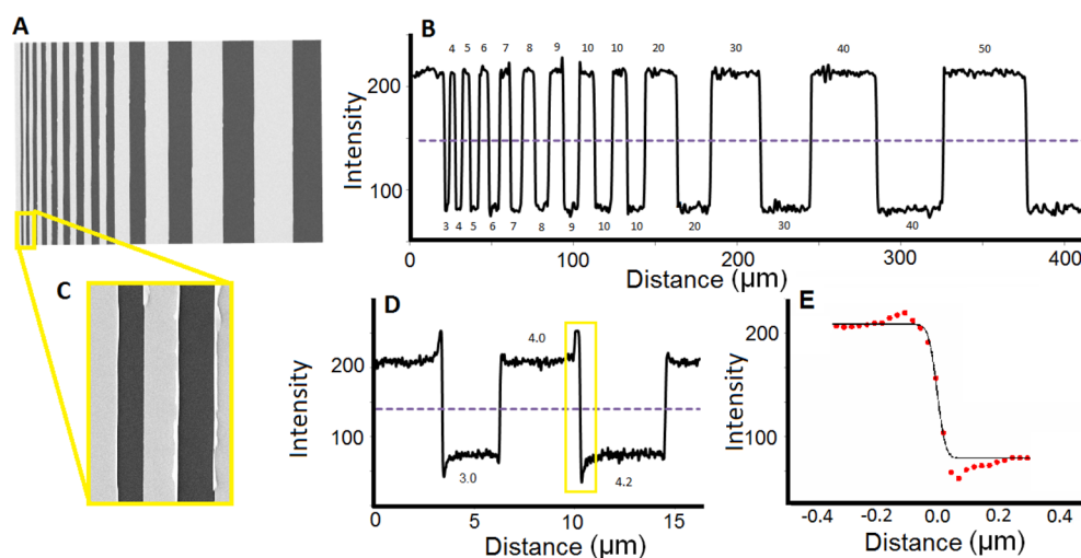
Figure 2. (A) SEM image of the unfunctionalized test device and (B) the corresponding linescan. (C) A zoomed-in SEM image of the 3 and 4 \mu\text{m} bars and (D) the corresponding linescan. (E) The sharp interface between the gold and silicon surface was fitted to the error function; the \Delta_{88\%-12\%} lateral resolution was measured to be 53 nm.
