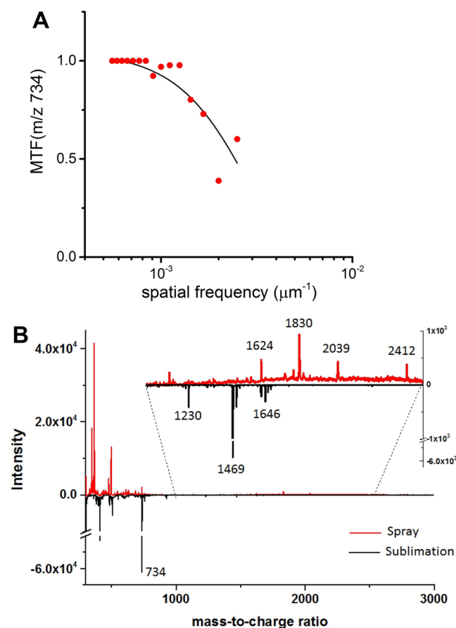
Figure 7. (A) The MTF for the protonated molecular ion of PC(16:0/16:0) at m/z 734.5 obtained after imaging the device using a solvent-based spray matrix application method (image step size: 50 \mu\text{m} ). (B) MALDI spectra from the device using the spray-based matrix application (top) and solvent-free sublimation method (bottom).
