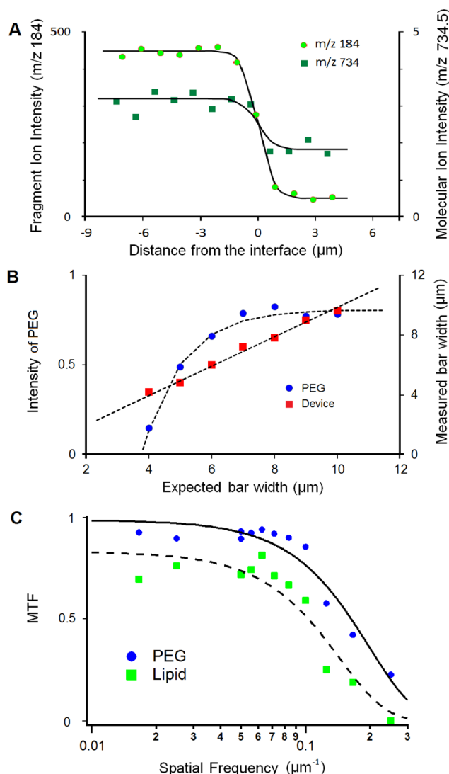
Figure 4. (A) Intensity of the molecular ion ( m/z 734 dark green) and fragment ion ( m/z 184, light green) signal of lipid, PC(16:0/16:0), at the chemical interface. Both traces were fit to the error function (solid line). (B) The normalized ion intensity of PEG ( m/z 107) plotted as a function of bar width (blue) and the linear relationship between the expected bar width and the measured bar width (red). (C) The MTF for PEG ( m/z 107, blue) and lipid ( m/z 184, green). Both traces were fit to a Gaussian function (solid line).
