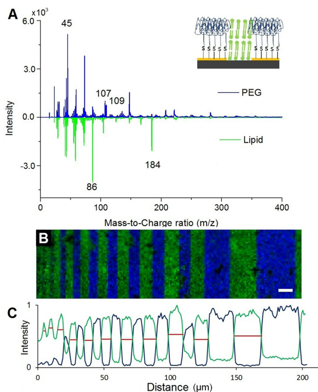
Figure 3. (A) Mass spectra obtained from the two distinct chemical regions of the device; the PEG (blue, top) and lipid (green, bottom) regions. (B) TOF-SIMS image showing the distribution of the PEG polymer fragments at m/z 45, m/z 107, and m/z 109 (blue) and lipid headgroup fragments at m/z 184 and m/z 124.9 (green). The scale bar is 10 \mu\text{m} . (C) The ion intensities for the PEG fragment ( m/z 107) and the lipid fragment ( m/z 184) were summed along the bar orientation and plotted as a function of lateral space. The fwhm for both the lipid (red) and PEG were measured and reported in Table S1 (see Supporting Information).
