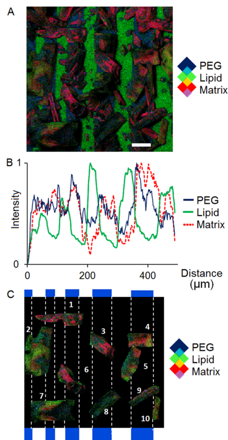
Figure 5. (A) TOF-SIMS image showing the distribution of matrix (red), PEG (blue), and lipid (green) after solvent-based matrix application (scale bar: 50 \mu\text{m} ). (B) The linescan of the three components demonstrates the mixing that occurs as a result of matrix application. (C) Ten individual matrix crystals were isolated from the ion image in order to emphasize the degree of chemical mixing and show the distribution of analyte molecules in matrix crystals.
