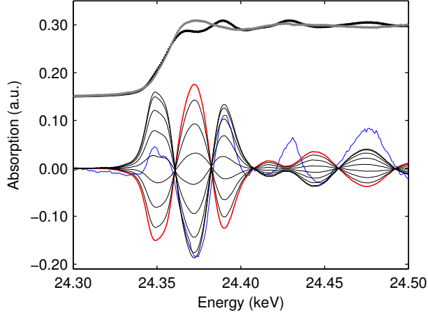
Figure 2: Demodulated spectra obtained from Pd/Al 2 O 3 at 400 °C ( \phi_k^{PSD} = 0\text{--}160^\circ ) together with scaled spectra of Pd foil and PdO powder. The red spectrum corresponds to \phi_k^{PSD} = 0^\circ and blue spectrum is the scaled difference spectrum Pd foil -PdO.
