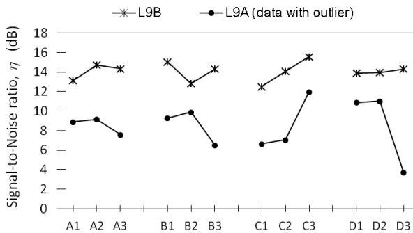
Figure 7 SNR factorial effect plot for L9B and L9A
