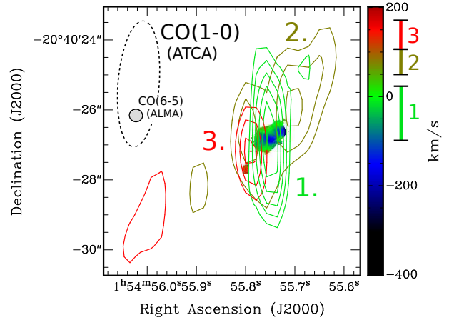
Fig. 4. Velocity map of CO(6–5) from Fig. 2 overlaid onto CO(1–0) contours, derived by integrating the CO(1–0) across the velocity ranges -100 - +20 \text{ km s}^{-1} (light-green #1), +50 - +110 \text{ km s}^{-1} (dark-green #2) and +110 - +170 \text{ km s}^{-1} (red #3) (EM15). Levels: 2.8, 3.5, 4.2, 4.9, 5.6, 6.3 \times \sigma ( \sigma = 12 \text{ mJy beam}^{-1} \times \text{km s}^{-1} for component #1 and \sigma = 7.3 \text{ mJy beam}^{-1} \times \text{km s}^{-1} for components #2 and #3). The color-codings of the CO(1–0) contours and CO(6–5) velocity map are closely matched.
