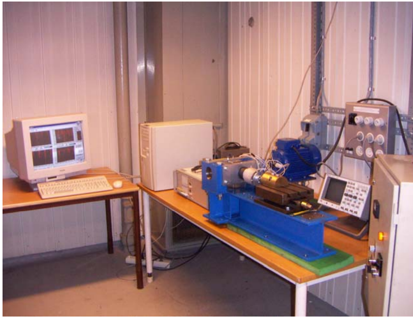
Figure 10. Setup for experimental study of performance of Chalmers Magnetostrictive Electric Generator.
