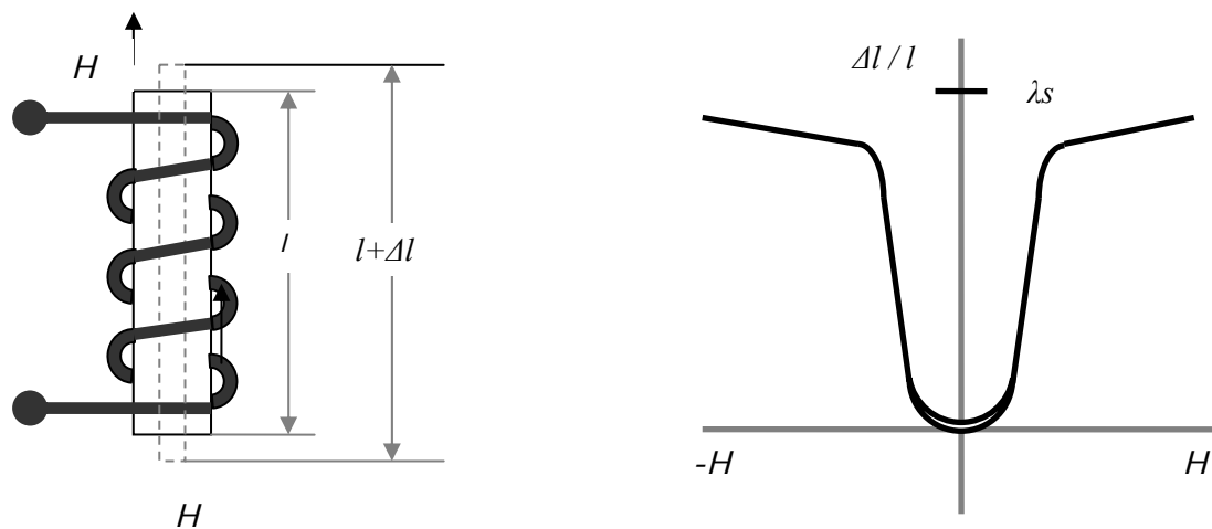
Figure 1. Schematic representation of the Joule effect.
