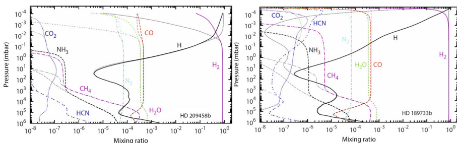
Fig. 6 Steady-state composition of HD 209458b (left) and HD 189733b (right) calculated with a non-equilibrium model (colour lines), compared to the thermodynamic equilibrium (thin black lines) [178]. For HD 189733b, one can clearly notice the higher sensitivity to photolyses and vertical mixing, with all species affected, except the main reservoirs, H_2 , H_2O , CO, and N_2 . Since the atmosphere of HD209458b is hotter, it is mostly regulated by thermochemistry. The EChO Origin survey would measure these differences by deriving the abundances of both key and minor molecular species, with mole fractions down to 10^{-5} to 10^{-7} (see Section 3.2.2 and 3.2.3)
