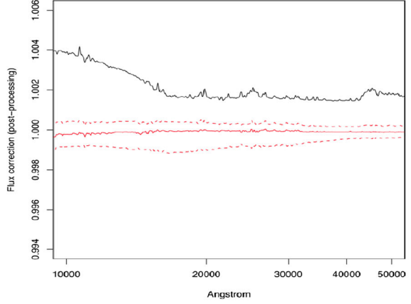
Teff=5200 - sigma= 500
