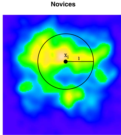
FIG. 11. The next fixation location is chosen from the black circle at distance l from the current fixation x_i according to the estimated intensity surface.
