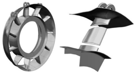
Figure 5. The TRS divided into segments, which are welded together in an assembly process.
