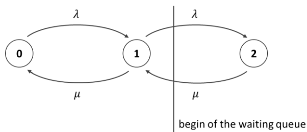
Figure 1: Transition graph of the queueing model.
