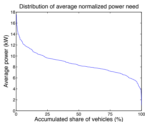
Figure 18: Average normalized power need. The power includes power need for overcoming rolling and air drag resistance and achieving the necessary acceleration and is for comparison normalized to properties of a midsize car (mass M = 1500 kg, air resistance C_d * A = 0.70 m 2 , and rolling resistance c_r = 0.01 .) (Source: Data Cars Corr 30d+ )
