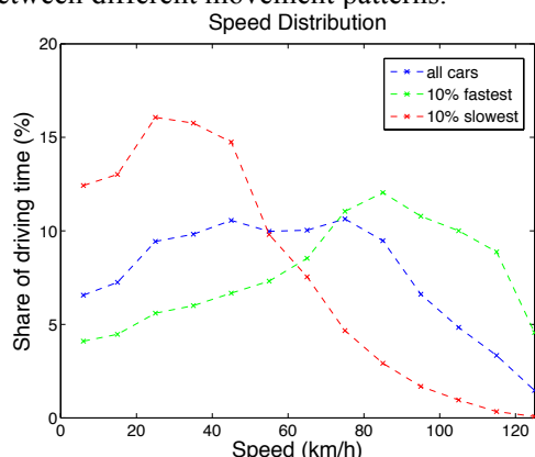
Figure 17: Speed distribution in 10 km/h intervals when driving, given as average values for all cars and for the deciles with the highest and lowest average speed, respectively. (Source: Data Cars Corr 30d+ )
