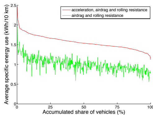
Figure 19: Vehicle average specific energy need at the wheel when driving \geq 2 km/h. The need is estimated as the sum of energy needs for overcoming rolling and air resistance and energy for achieving the positive acceleration. For comparison of movement patterns, the energy need is for all the vehicles normalized to the properties of an assumed midsize car (mass M = 1500 kg, air resistance C_d * A = 0.70 m 2 , and rolling c_r = 0.01 .) (Source: Data Cars Corr 30d+ )
