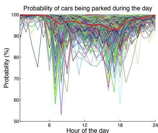
Figure 14: Probability for the logged individual cars of being parked for different hours of the day. The thicker red line denotes fleet average. Source: Data Cars 30d+ .
