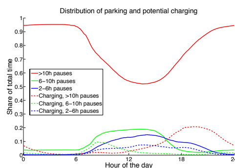
Figure 16: The distribution in time for parking of different lengths and as illustration possible charging during these pauses. Presented as shares of total measurement time for the vehicle fleet. Assumed charging: PHEVs with 2 kW charging immediately after parking which continues until battery is full (10 kWh) or pause ends. Energy use 0.2 kWh/km in CD mode. Source: Data Cars Corr 30d+ .
