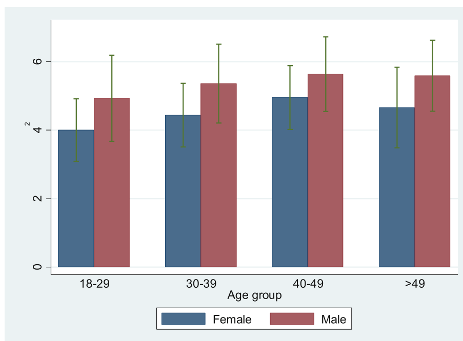
Fig. 1 Diet-related greenhouse gas emissions by age and gender in the LifeGene study, 2009–10, Sweden ( n = 5,364 ). The distribution of crude median and IQR of daily diet-related greenhouse gas emissions expressed as kg CO 2 e by age and gender
