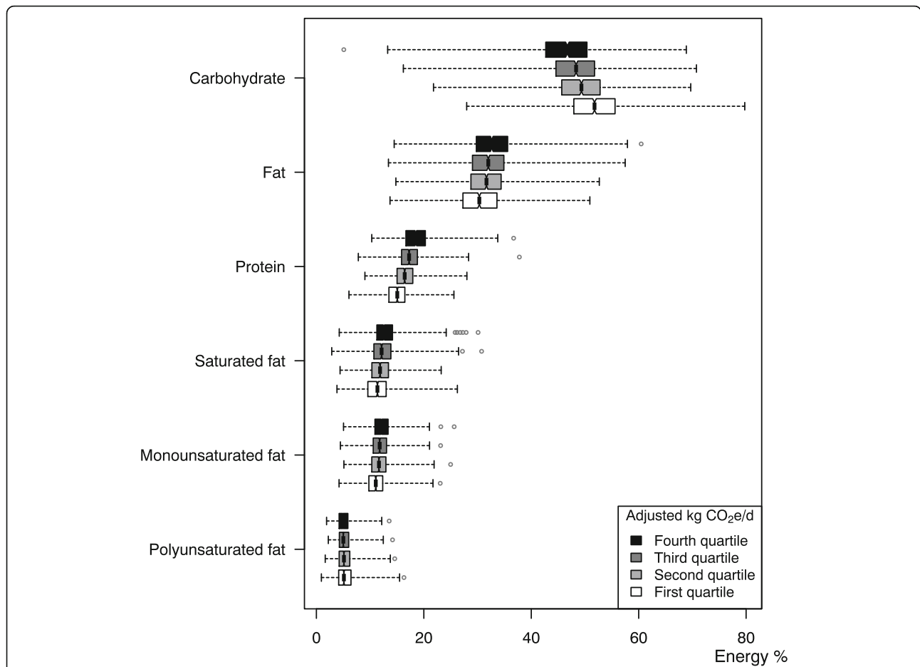
Fig. 2 Percentage of energy coming from macronutrients by quartiles of increasing levels of greenhouse gas emissions in the LifeGene study, 2009–10, Sweden ( n = 5,364 ). The percentage of energy coming from fat, protein, carbohydrates, saturated fat, monounsaturated fat, and polyunsaturated fat, respectively, by quartiles of increasing levels of energy adjusted diet-related greenhouse gas emissions
