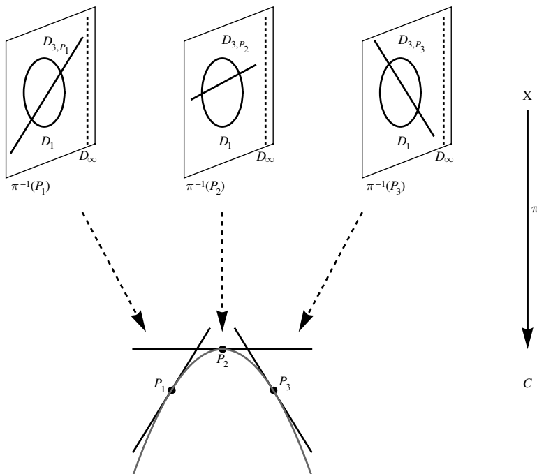
FIGURE 2. Fibered threefold
