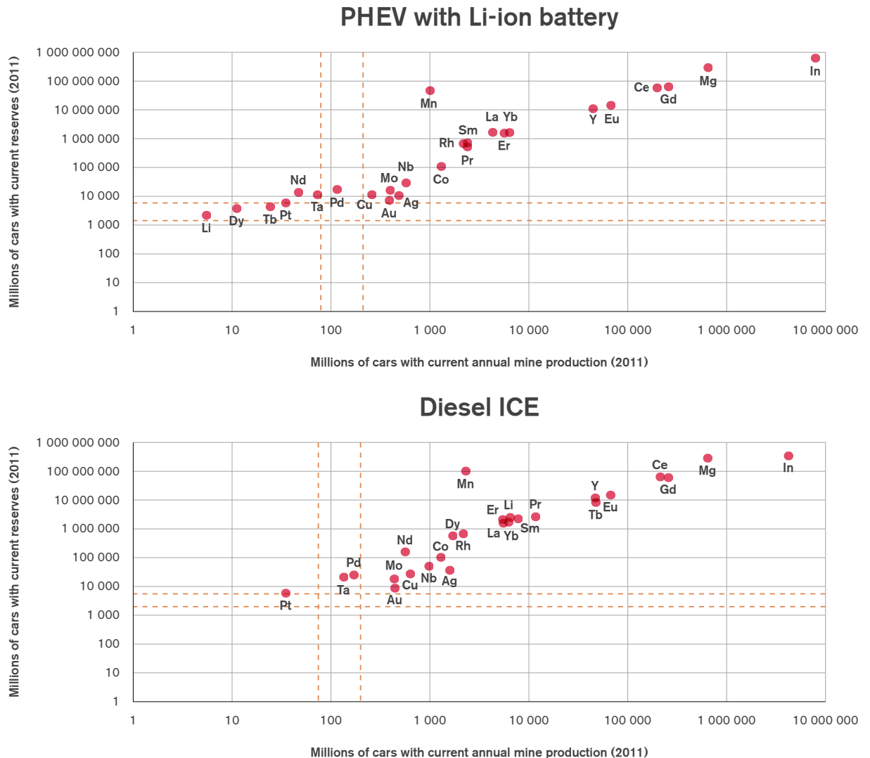
Figure 7.5 Comparison of metal requirements for a PHEV with Li-ion battery and a diesel ICE (both in the executive compact family car segment, see Table 6.2). The diagrams show, for each car, the maximum number of cars that the current reserves would allow (y-axis) and the maximum annual growth rate of the vehicle fleet that the current annual resource extraction would allow (x-axis), if, hypothetically, each metal would be used only for passenger cars and if there were no material losses. Note that reserves data can differ between sources, e.g. REE (a factor of 2) and indium (a factor of 10), and for the purpose of this analysis, low reserve estimates were chosen 19 .
