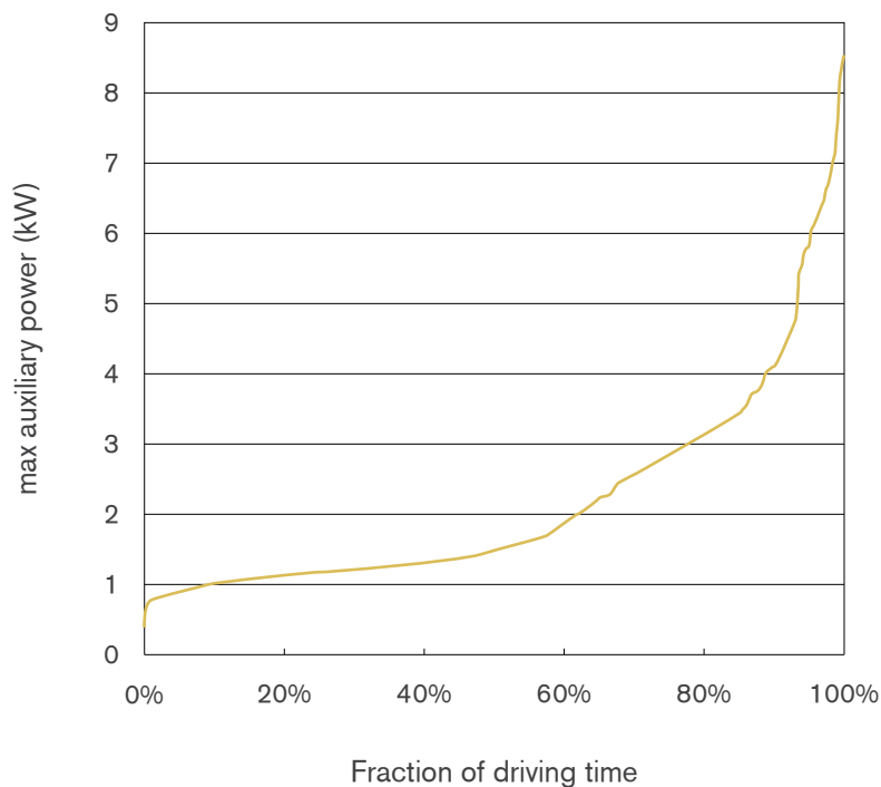
Figure 5.5 Measured auxiliary power use in six Peugeot Ions during real driving. The driving occurred at all seasons
