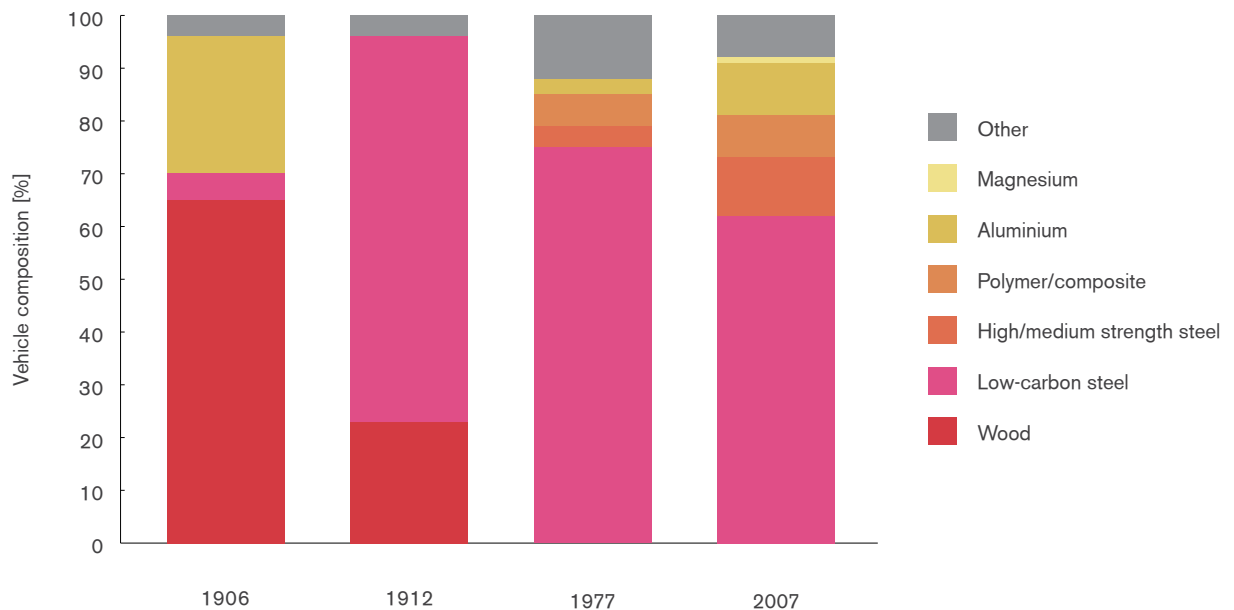
Figure 7.3 Historical shift in car composition by mass. 14
