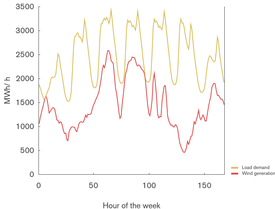
Figure 9.1 Weekly load demand and wind generation fluctuation sample data from Western Denmark. The intermittent variation of the wind output is seen to be uncorrelated to the daily load variations, which can thus reduce reliability and efficiency of the electricity system.
