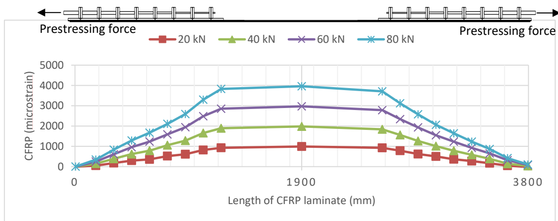
Figure 4. Tensile strain in CFRP laminate under prestressing force up to 80 kN in specimen B3
