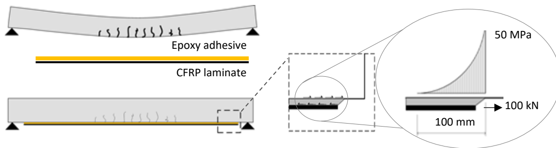
Figure 2. Interfacial shear stress concentration developed at each end of CFRP laminate upon releasing of prestressing force (Haghani and Al-Emrani, 2016; Haghani et al., 2009)
