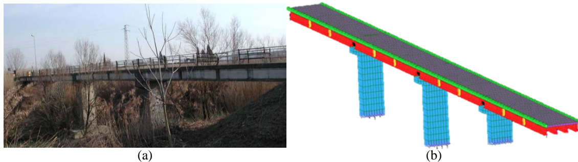
Figure 5. (a) Side view of the San Miniato bridge; (b) Finite element model of the San Miniato bridge
