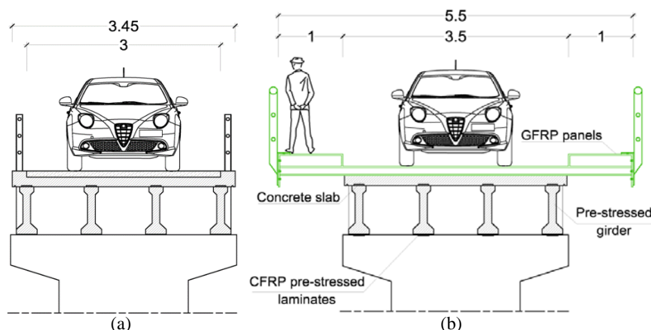
Figure 6. (a) Existing cross section, (b) widened cross section.
