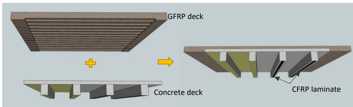
Figure 1. SUREBridge concept—externally bonded (EB) prestressed CFRP laminates on the bottom of girder (tensile part) and GFRP panels on the top of the existing concrete deck (compressive part)
