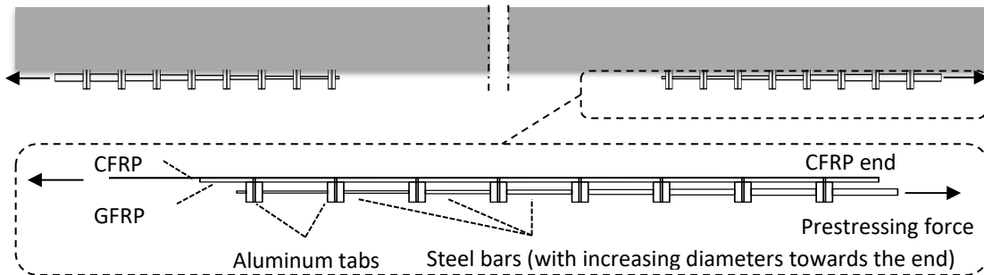
Figure 3. Applying stepwise prestressing force in CFRP laminate using the new technique
