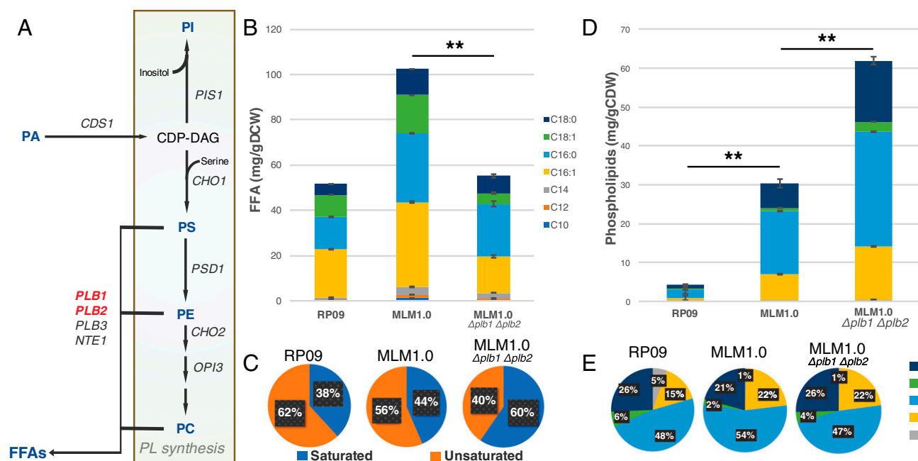
Fig. 4. Effect of deleting phospholipase genes PLB1 and PLB2 on FFA production. (A) Role of phospholipases B in FFA formation in MLM1.0. Signaled in red are the genes PLB1 and PLB2 that were deleted to validate this hypothesis. (B) Total FFA quantification of MLM1.0 with PLB1 and PLB2 being deleted compared with strains MLM1.0 and RP09. (C) Distribution of saturated and unsaturated C16 and C18 FFAs in the three strains. (D) Phospholipid levels in strains RP09, MLM1.0 and MLM1.0 + \Delta plb1 \Delta plb2 . PC, phosphatidylcholine; PE, phosphatidylethanolamine; PI, phosphatidylinositol; PS, phosphatidylserine. (E) Phospholipid classes distribution in strains RP09, MLM1.0 and MLM1.0 + \Delta plb1 \Delta plb2 . Strains were grown for 72 h in minimal medium containing 2% glucose, FFA and total lipid quantifications were performed with five biological replicates. ** P < 0.005 (Student's t test: two-tailed, two-sample equal variance).
