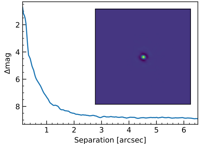
Figure 5. The I band image of K2-136 (inset, 3'' \times 3'' ) from NOT/FastCam and resulting 5- \sigma contrast curve. North is up and east is to the left.
