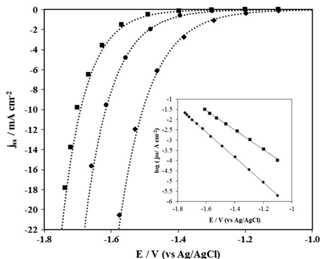
Fig. 7 Steady-state current measurements (symbols) and simulated irreversible one-electron transfer (dotted line). Inset shows the Tafel plots for the j_{ss} experiments. Bare Ti (dots), \text{Cr}(\text{OH})_3 @Ti (squares), and \text{Cr}_2\text{O}_3 @Ti (diamonds)
