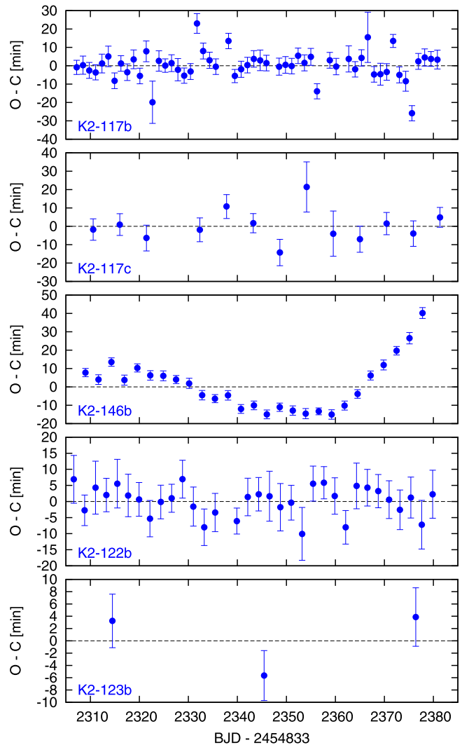
Figure 9. O - C diagrams for mid-transit times for K2 campaign field 5 planets.
