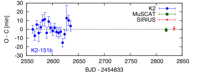
Figure 16. O - C diagram for mid-transit times for K2-151b. Ground-based transit observations are shown by the green square (MuSCAT) and red triangle (SIRIUS).
