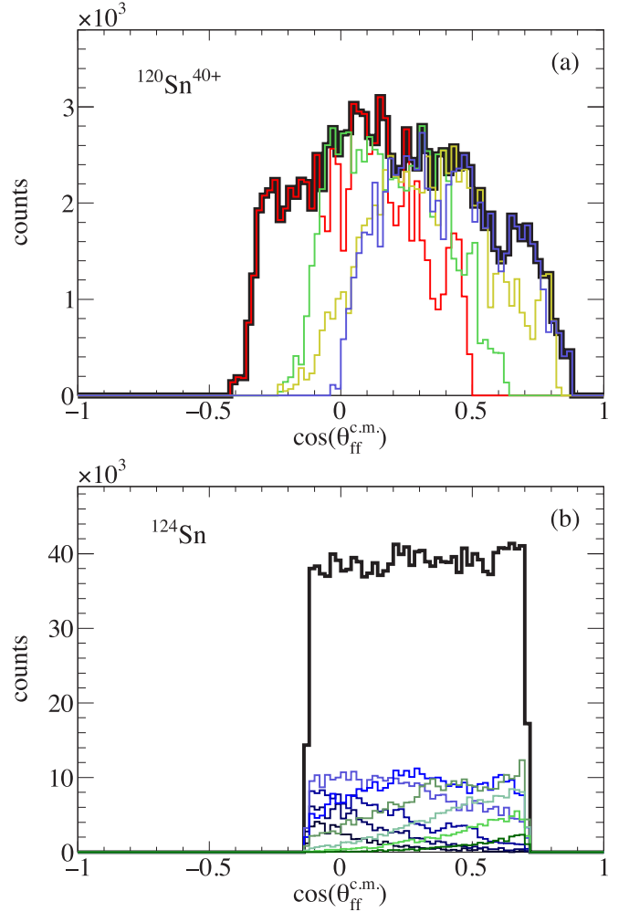
FIG. 9. (a) \cos(\theta_{ff}^{c.m.}) distribution of the charge state q = 40 of ^{120}\text{Sn} . The contributions of the four settings of VAMOS are represented in color. The envelope distribution depicts the total distribution. (b) The full \cos(\theta_{ff}^{c.m.}) distribution of ^{124}\text{Sn} within the VAMOS acceptance is presented in black, while the contribution of each q is presented in color.
