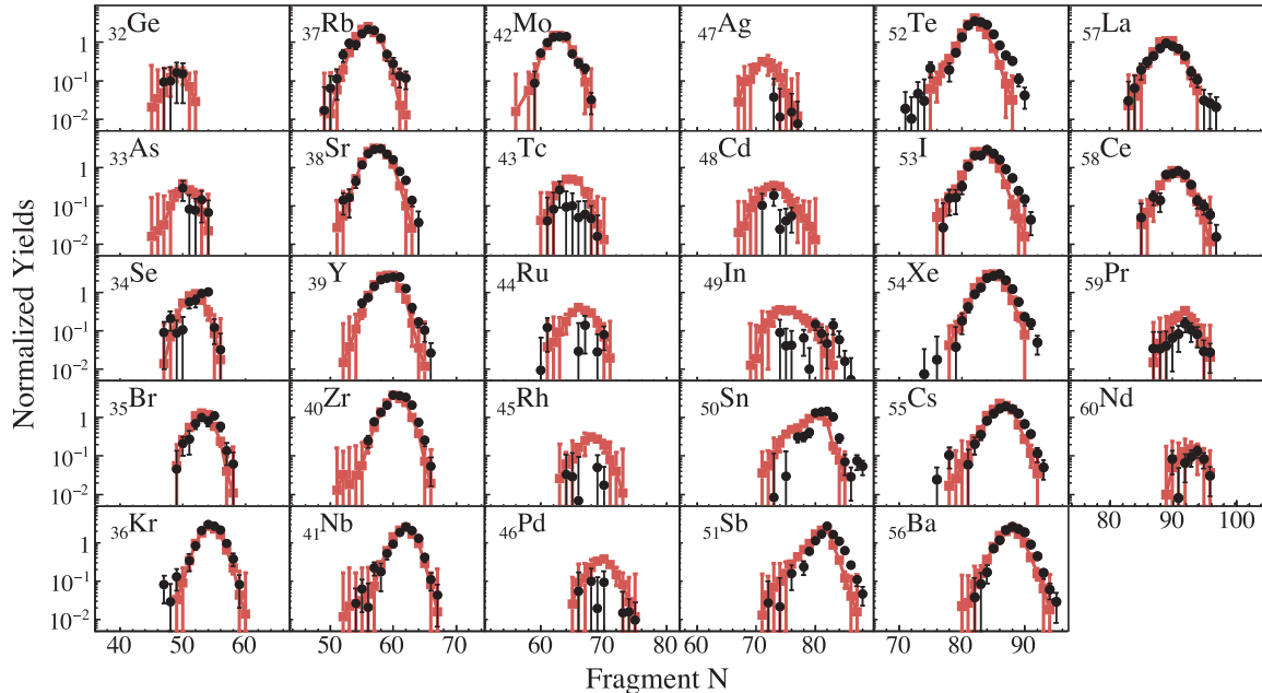
FIG. 11. Isotopic fission-fragment yields of ^{238}\text{U} ( \langle E_x \rangle = 7.4 MeV). Present data (in black) are compared with data from Coulomb-induced fission [13] (in red).
