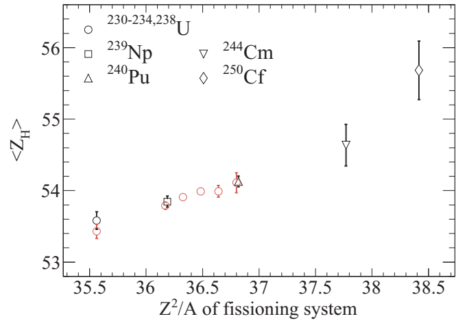
FIG. 18. Average Z value of the heavier fragment in the asymmetric fission as a function of the fissility parameter. Present data (in black) are compared with previous measurements of several U isotopes [1,13] (in red).
