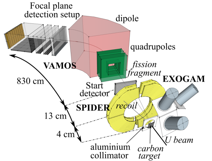
FIG. 1. Experimental setup scheme. The thick black line on the right side represents the beam impinging on the target. A transfer reaction is shown followed by a fission decay; the three thin lines represent the target-like recoil and the two fission fragments. The recoil is stopped in the SPIDER detector while one of the fission fragments triggers the start detector and passes the VAMOS spectrometer before being measured with the focal-plane detection setup. The EXOGAM detector, for \gamma -rays measurements, is also shown surrounding the target (for clarity, only three EXOGAM clovers are indicated).
