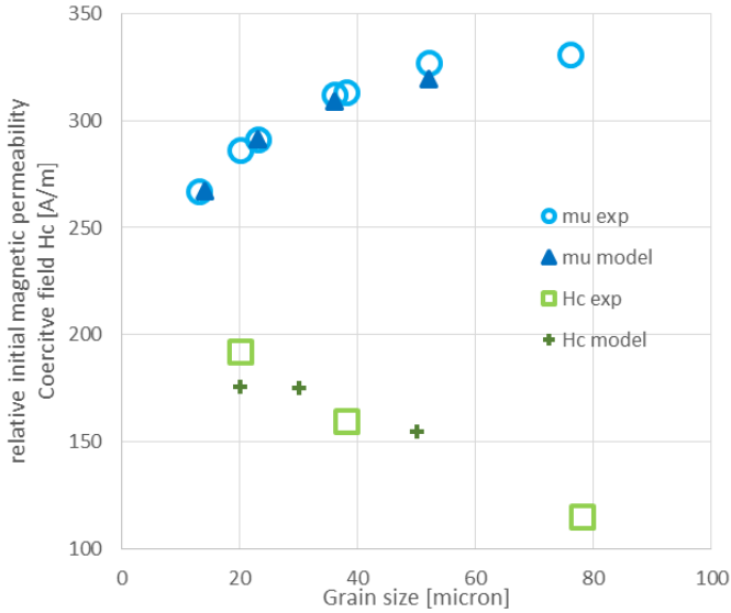
Figure 7. Model and experimental results for the initial magnetic permeability ( \mu ) and coercive field H_c as a function of the grain size, for a fully recrystallised low carbon steel.
