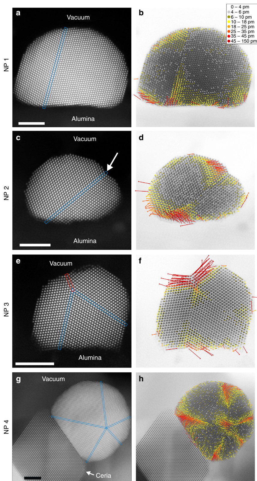
Fig. 1 High-precision atomic-resolution STEM images and displacement maps of supported Pt NPs. Left column, a , c , e and g : High-precision side-view HAADF STEM images of Pt NPs along \langle 110 \rangle supported on alumina ( a , c , e ) and ceria ( g ). The interfaces between the NPs and the support are seen at the lower edge of the NPs. The arrow in c marks a concave re-entrant surface. Right column, b , d , f and h : Displacement maps showing the deviation of each atomic column position from their unstrained lattice positions. The arrows display the direction and magnitude of each displacement, as indicated in the legend. Each scale bar corresponds to 3 nm
