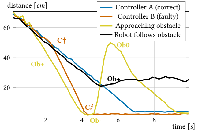
Figure 7. Controller sandbox, real robot: correct controller approaching a stationary obstacle, faulty controller approaching a stationary obstacle, obstacle approaches robot, and robot follows a moving obstacle. Ob^+, Ob^0, Ob^- indicate proceeding, stopped, and receding obstacles, respectively.
