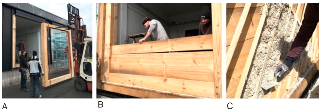
Figure 5. Construction of two full-scale test walls at Lund University, A) Construction of post-and-plank walls, B) Timber planks mounted between the posts, C) Application of hemp-lime on the post-and-plank wall. Photos: Paulien Strandberg.
