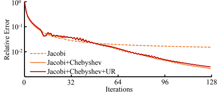
Fig. 6. The effect of under-relaxation (UR) on the armadillo example. This plot shows that under-relaxation has limited influence on the convergence of the Chebyshev approach, when \gamma = 0.9 .
