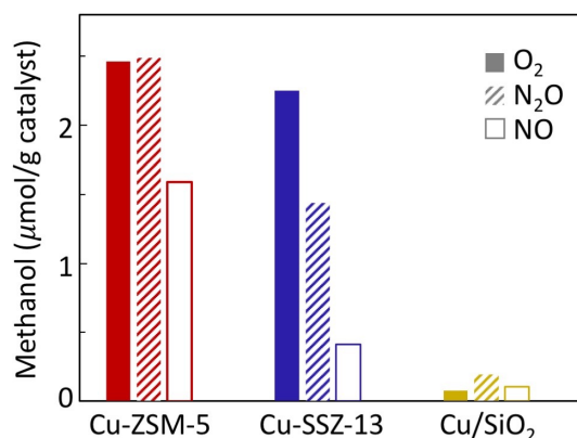
Figure 1. Methanol production over Cu-ZSM-5, Cu-SSZ-13 and Cu/SiO 2 at 1 atm using O 2 , N 2 O or NO as oxidants.
