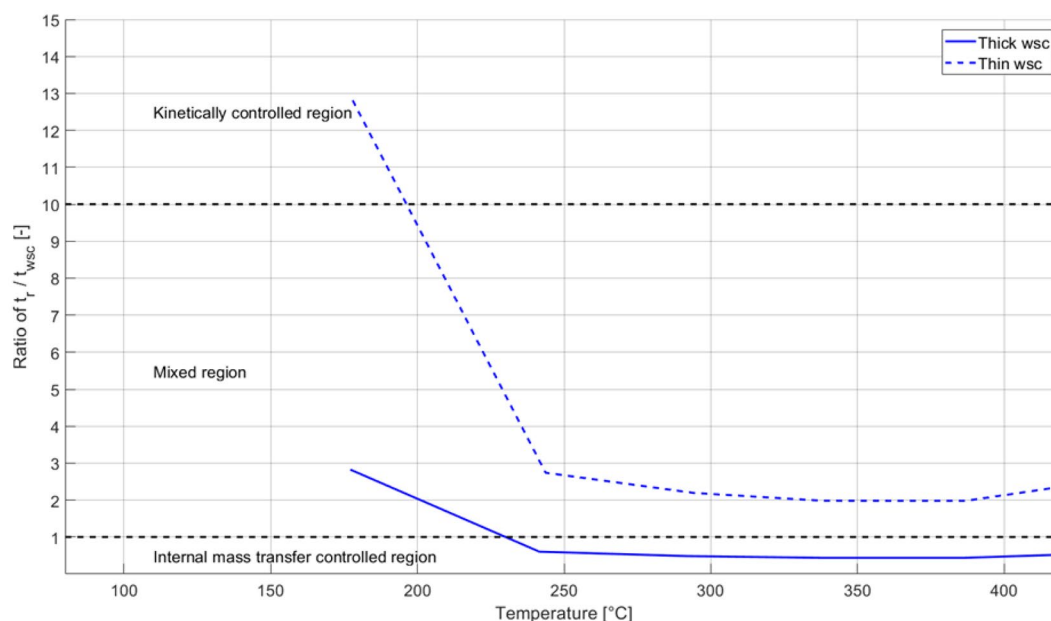
Fig. 4 Ratio of reaction time constant to washcoat diffusion time constant. Blue solid and dotted line correspond to thick and thin washcoat, respectively. Three control regions; kinetically controlled, mixed
