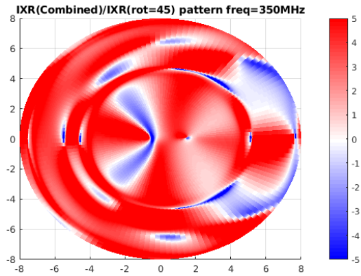
Figure 5: IXR(Combined)/IXR(rot=45) in dB. The mostly positive dB regions indicates that the IXR of the combined configuration is generally better than the rotation 45 configuration alone. Note that the orientation of x,y are flipped here with respect to Figure 1.
