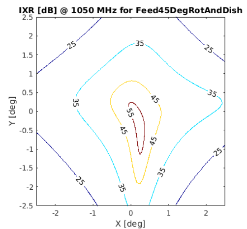
Figure 3: Contour map of IXR pattern of band 1 feed with rotation 45 at 1050 MHz. Contour lines are marked in units of dB. Note that the orientation of x,y are flipped here with respect to Figure 1.
