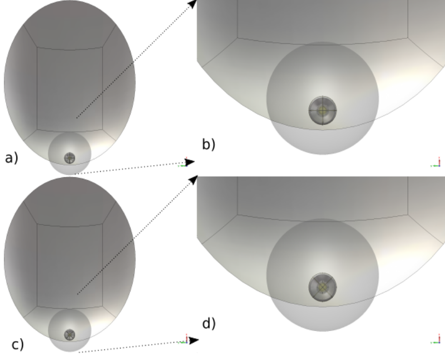
Figure 1: Overview of the two feed configurations showing the main reflector, the secondary reflector and the QRFH feed placement. b) & d) are zoom-ins of a) & c) respectively. As can be seen in b) & d), the only difference in the configurations is the rotation of the feed. The alignment of the linear feed probes are the same as the ridges seen as a cross at the center of the feed. a) & b) show the rotation 0 alignment while c) & d) show the rotation 45 alignment. The coordinate system is x pointing straight up while y is pointing to the left.
