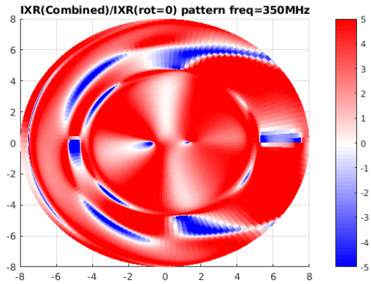
Figure 4: IXR(combined)/IXR(rot=0) in dB. The mostly positive dB regions indicates that the IXR of the combined configuration is generally better than the rotation 0 configuration alone. Note that the orientation of x,y are flipped here with respect to Figure 1.
