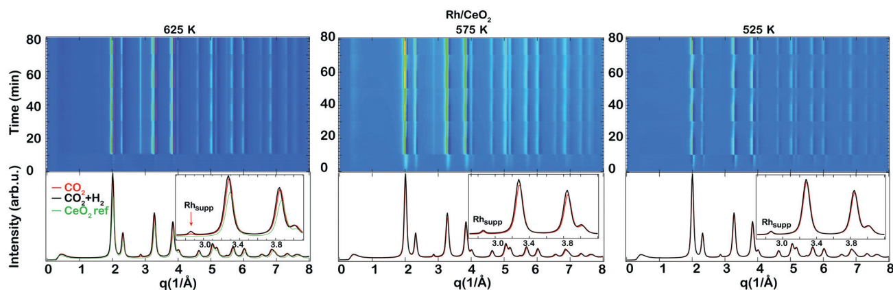
Fig. 3 X-ray diffractograms during transient hydrogenation of 0.5 vol% CO 2 over the as-prepared Rh/CeO 2 catalyst during periodic variation of the feed gas composition between 2 vol% H 2 + 0.5 vol% CO 2 and 0.5 vol% CO 2 at 625, 575 and 525 K for 10 min recorded using HE-XRD. The top panel shows the color coded intensities of the XRD patterns in the 0–8 Å -1 region versus time. The bottom panel shows selected XRD patterns at the end of selected CO 2 (red) or CO 2 + H 2 (black) pulses together with the pattern recorded from the ceria reference sample (green). The inset indicates a zoom in between 2.7 and 4.1 Å -1 .
