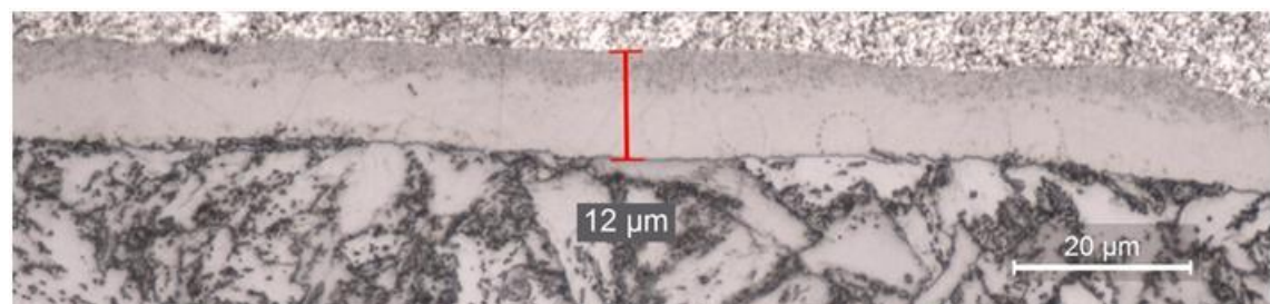
e) Reamed
