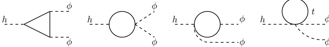
FIGURE 2 | Leading contributions to the decay h \rightarrow \phi\phi .
