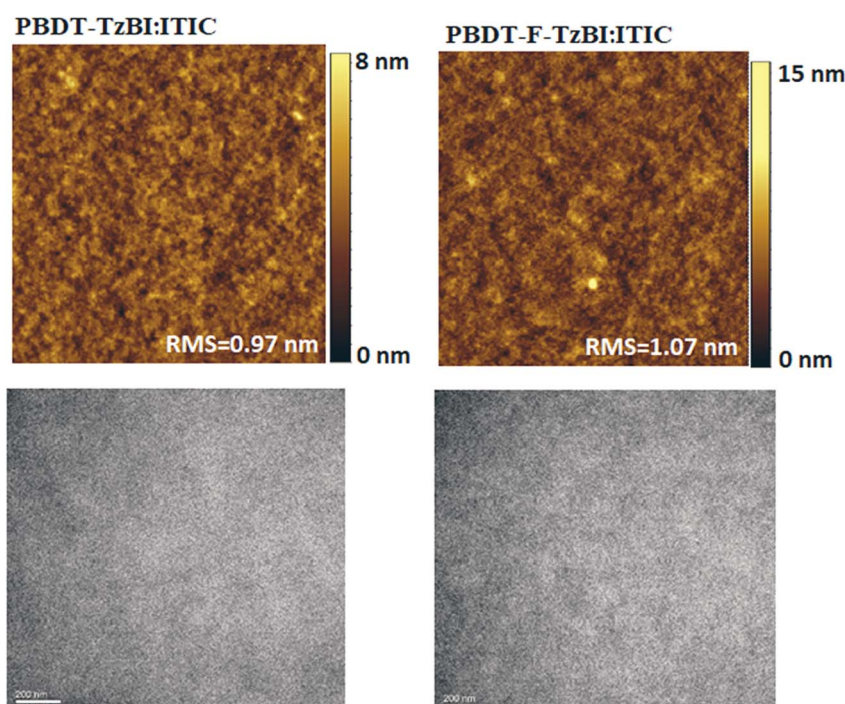
Fig. 3 AFM topography ( 5 \times 5 \text{ nm} ) and TEM images of the optimized PBDT-F-TzBI:ITIC and PBDT-TzBI:ITIC blend films.
