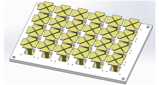
Fig.4. 24-element C-band phased array feed model
