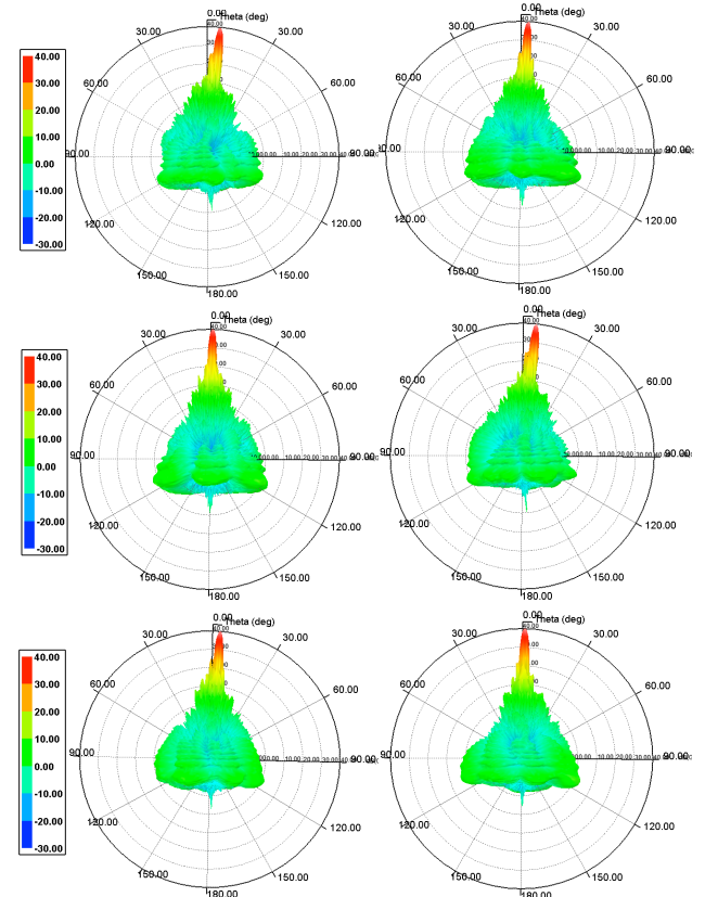
Fig.5. Secondary radiation pattern of a quarter of the array (corresponding to 6 array elements in the first quadrant on the top left of the array)
