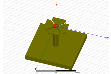
Fig. 1. Geometry of the tightly fed Bowtie antenna.
