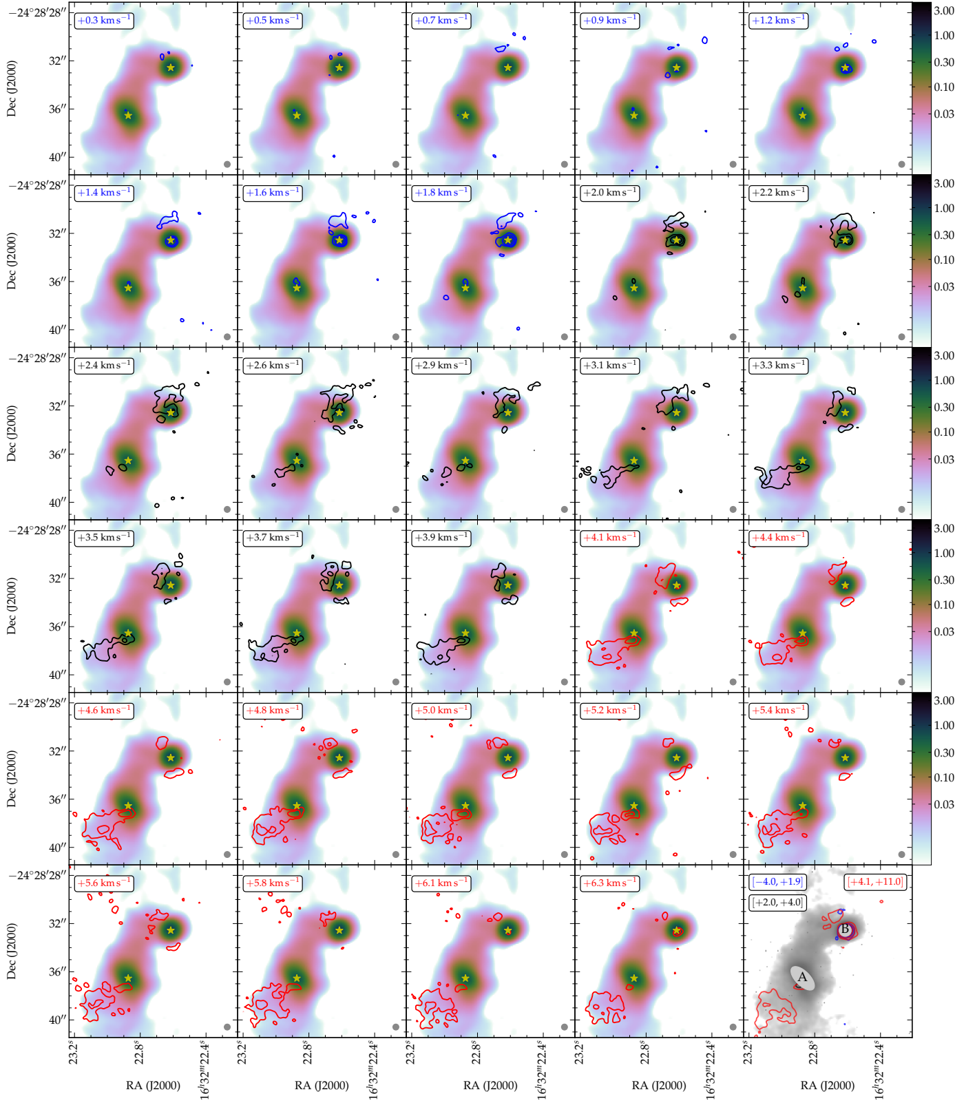
Fig. B.7. 29 SiO 8–7 channel maps. As Fig. B.1. First positive (negative) contour level in individual channel maps: 0.02 (–0.04) Jy beam -1 ; first contour levels in the bottom right integrated ranges panel: 0.07 Jy beam -1 km s -1 .
