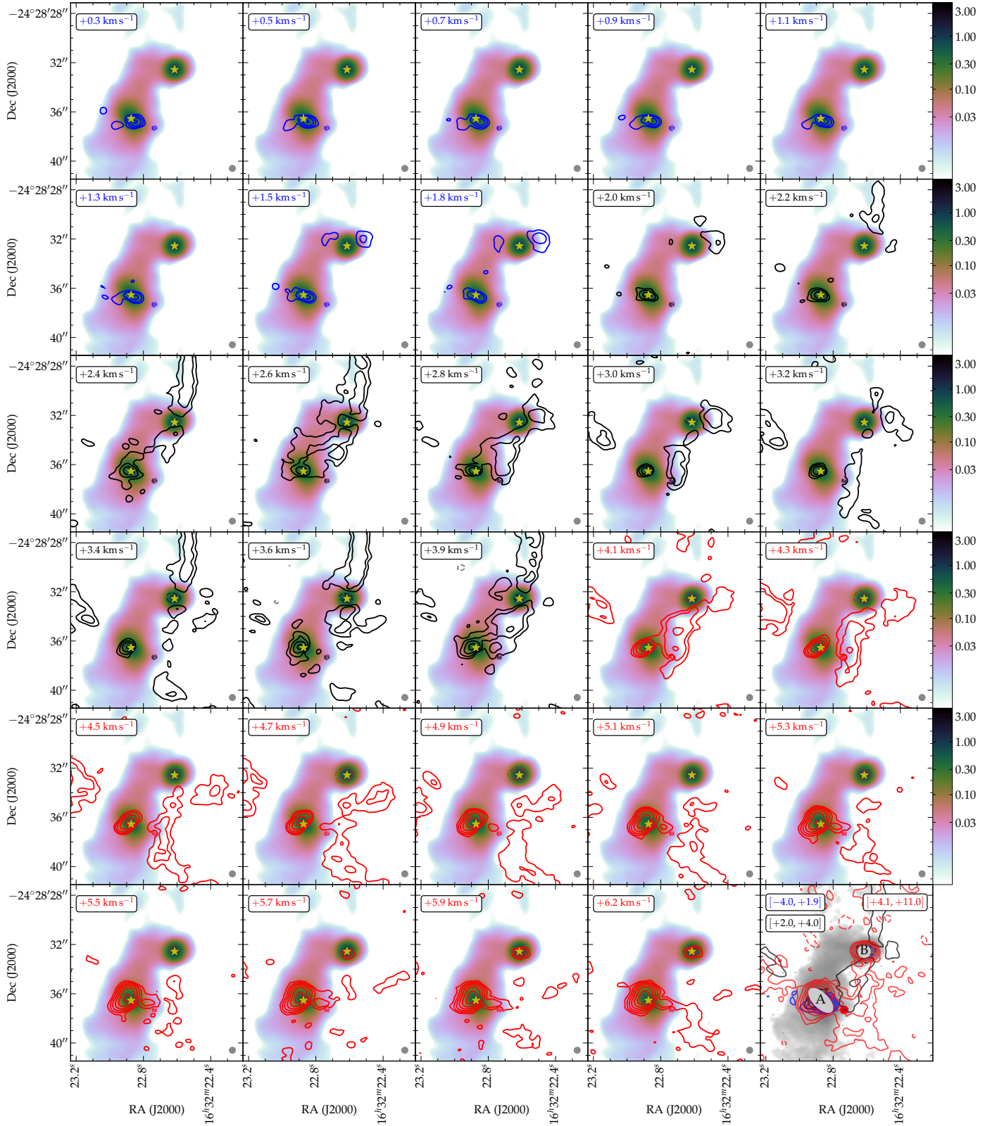
Fig. B.8. \text{C}_2\text{H} channel maps. As Fig. B.1. First positive (negative) contour level in individual channel maps: 0.03 (−0.06) Jy beam −1 ; first contour levels in the bottom right integrated ranges panel: 0.07 Jy beam −1 km s −1 . Note that emission in channels above +5 km s −1 is due to \text{CH}_3\text{CN } 19(3)-18(3) and not \text{C}_2\text{H} .
