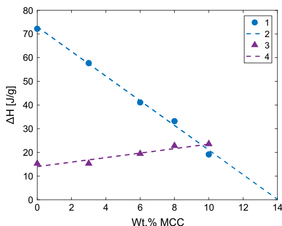
Fig. 3 Enthalpy of TMAH-hydrate (1) with linear trendline (2) and NaOH-hydrate (3) with linear trendline (4) as a function of cellulose concentration in solutions of 2.3 M 50/50 mol% NaOH/TMAH(aq)
