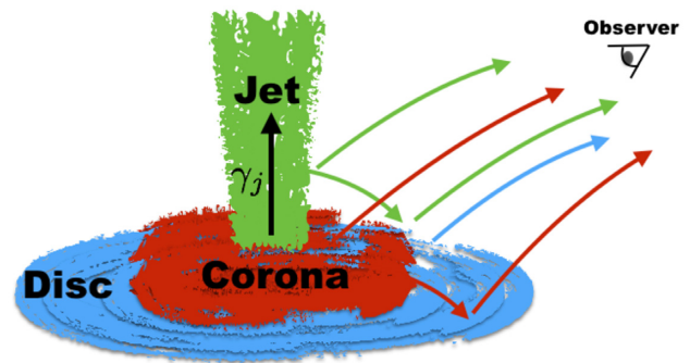
Figure 7. Diagram of a corona+jet model for a BHB, representing spectral Model B2. The thin disc is truncated to radii on the order of 2–10 r_g , and an optically thin compact corona exists within the inner accretion flow, with electron temperatures kT_e \sim hundreds of keV. The jet electrons are relativistic, with kT_e \geq 511 keV, and the plasma has bulk motion in the z -direction with \gamma_j \sim on the order of 1 to a few. The observer sees emission from the jet in the form of synchrotron, SSC, and IC scattering of disc photons, as well as IC emission from the corona, and blackbody emission from the disc. The jet and coronal X-ray components irradiate the disc, resulting in a reflected X-ray spectrum.
