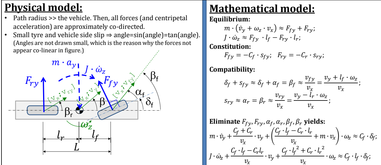
Figure 4-44: Less general derivation of the Linear 1-Track Model, i.e. Eq [4.50].
