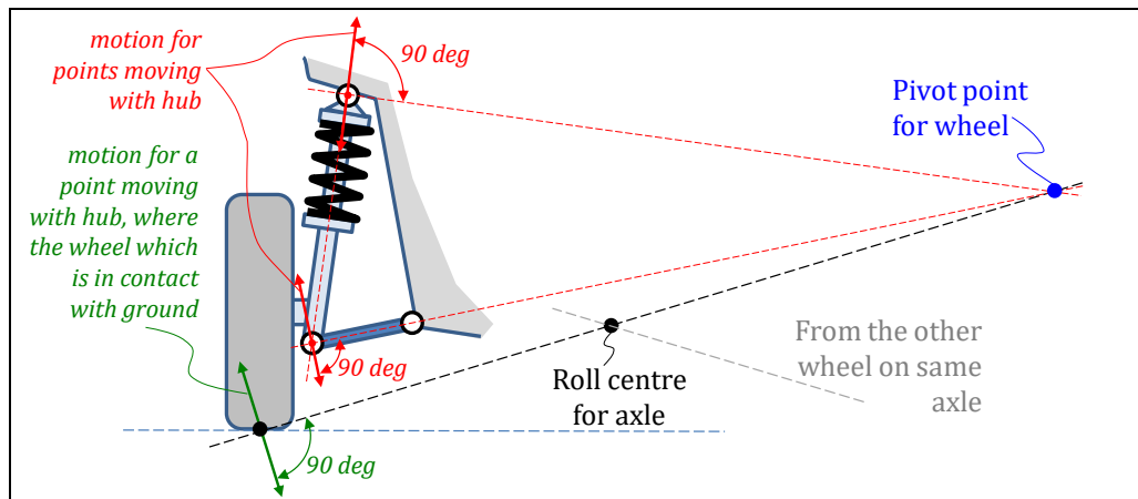
Figure 2-58: Example of how to appoint the pivot point for one wheel, and roll centre height, for axle with double McPherson suspension.
