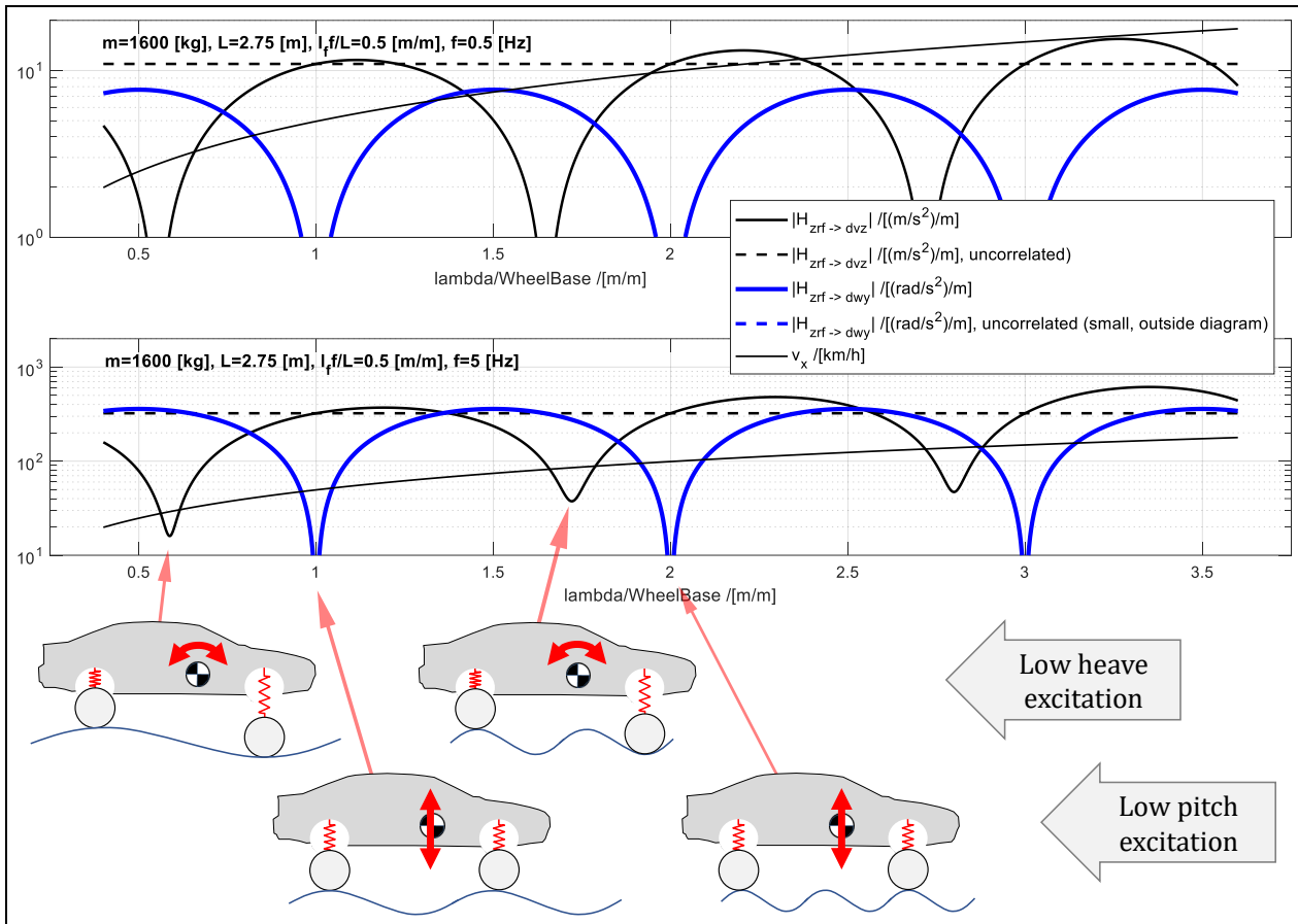
Figure 5-30: Wheel Base Filtering, as compared to “uncorrelated”. Response |H_{zrf \rightarrow vzg}| and |H_{zrf \rightarrow \omega y}| . Two frequencies, 0.5 and 5 Hz. Varying Road Wavelengths, so also v_x has to vary.
