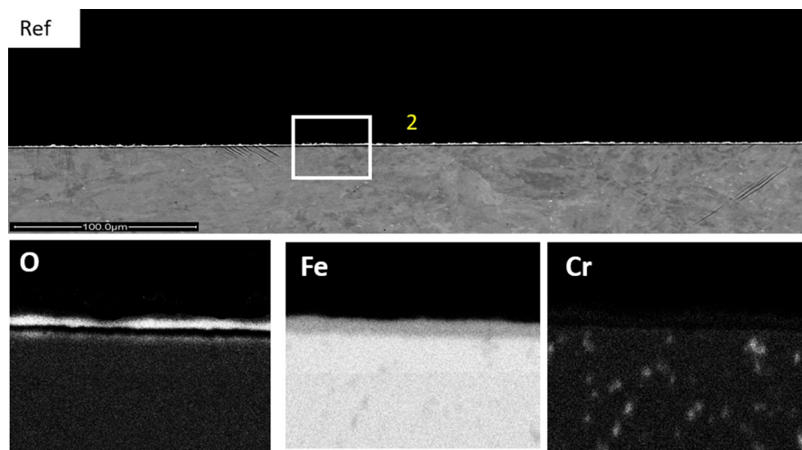
Fig. 7 BIB cross section SEM/EDX maps of Fe-2.25Cr-1Mo after 24 h at 400 °C in 5% O 2 + 20% H 2 O + 75% N 2 (higher-magnification image of an area in Fig. 7a)
