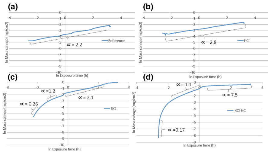
Fig. 3 \ln(m) versus \ln(t) of TG mass gain curves of Fe-2.25Cr-1Mo steel at 400 °C in 5% \text{O}_2 + 20% \text{H}_2\text{O} + 75% \text{N}_2 , a reference, b with 500 vppm \text{HCl(g)} , c with \text{KCl(s)} , d with \text{KCl(s)} - 500 vppm \text{HCl(g)} . The first 5 min of data in the TG exposures were of relatively poor quality due to the rapid heating and are therefore excluded
