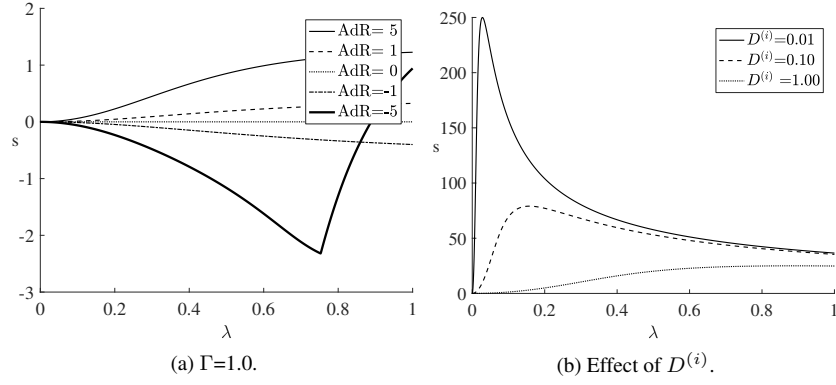
Figure 16: s versus \lambda for different values of parameters.
