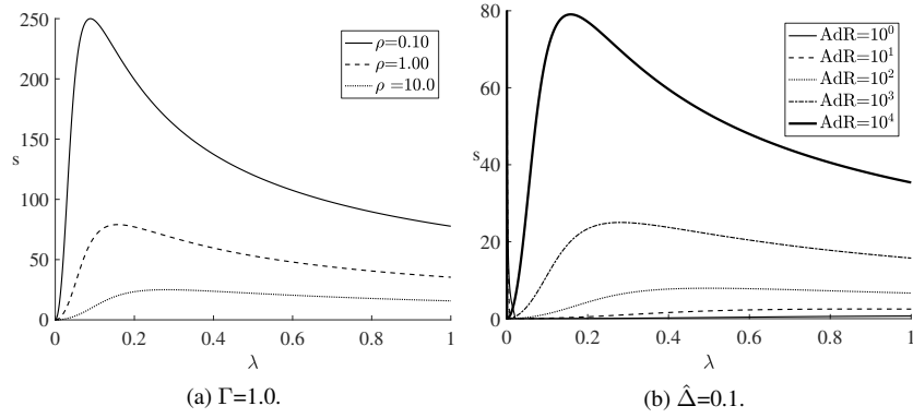
Figure 17: s versus \lambda for different values of \hat{\alpha} and \hat{\Delta} .
