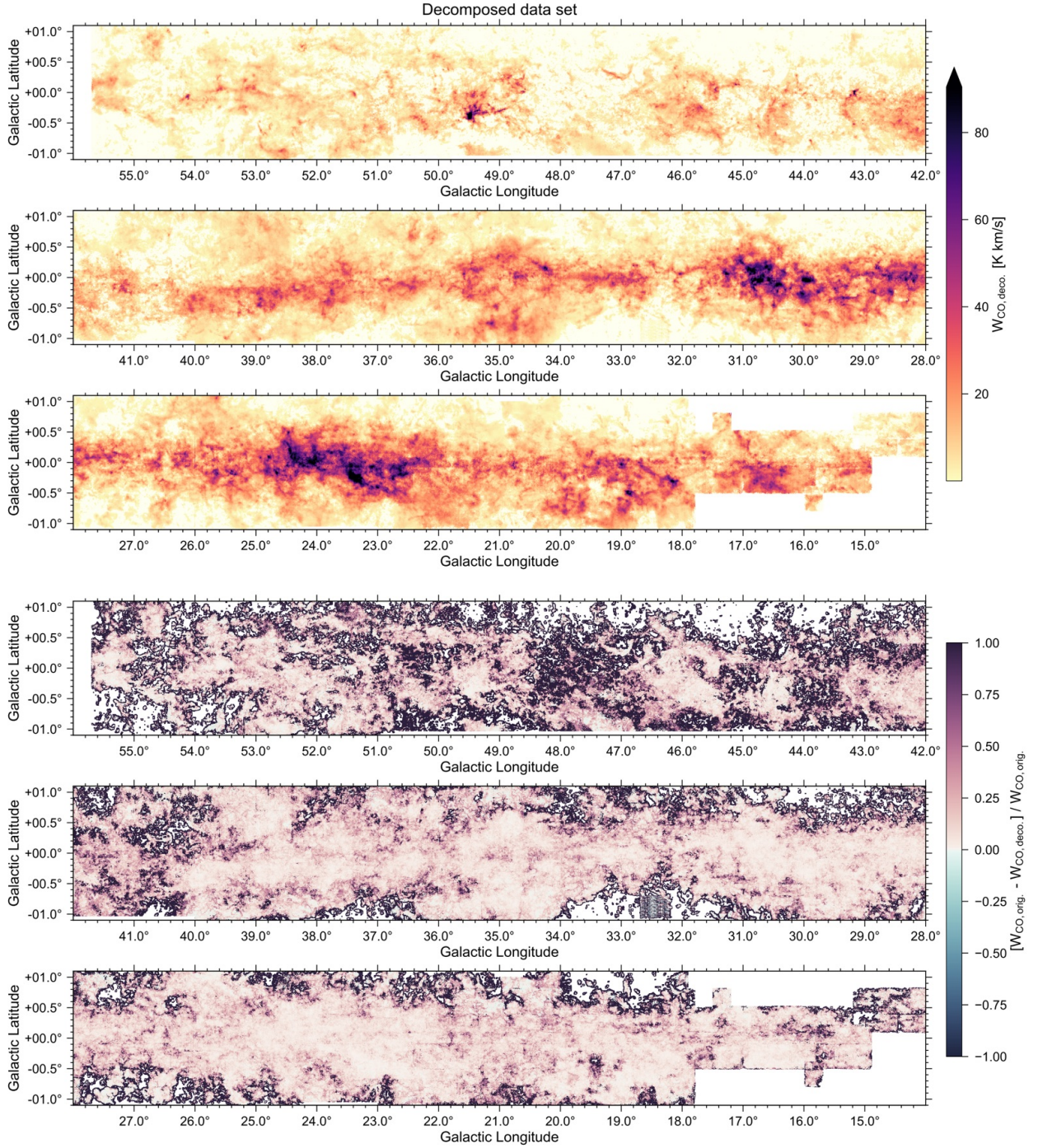
Fig. 2. Top: zeroth moment map of the GRS data set recreated from the Gaussian fit components and integrated over the entire velocity range ( -5 \lesssim v_{LSR} \lesssim 135 \text{ km s}^{-1} ). When displayed in Adobe Acrobat, it is possible to switch to the map of the original data set . Bottom: map of the normalised residual values.
