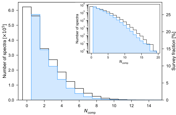
Fig. 5. Histogram of the number of fitted Gaussian components per spectrum across the whole GRS data set for the full decomposition results (black line) and the fit components with S/N > 3 (blue). The inset shows the same distribution on a logarithmic scale.
