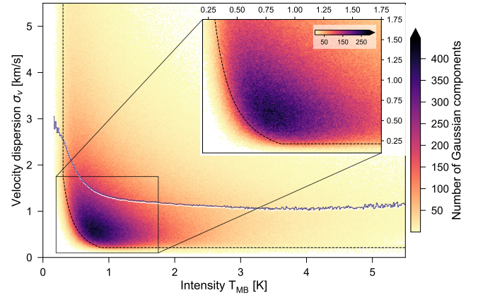
Fig. 9. 2D histogram of intensity and velocity dispersion values for all fit components. The dashed line shows the lower limit for a chosen significance value of S_{\text{min}} = 5 and a velocity dispersion value corresponding to the spectral resolution limit of the survey ( 0.21 \text{ km s}^{-1} ). The blue line shows the mean \sigma_v value per intensity bin. The number of bins in either direction is 400. The inset is a zoom-in of the most dense region of the distribution and uses a finer grid with 175 bins in either direction.
