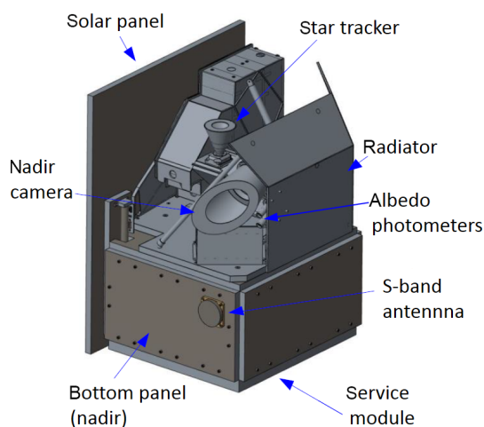
Figure 2. Layout of the MATS satellite.
