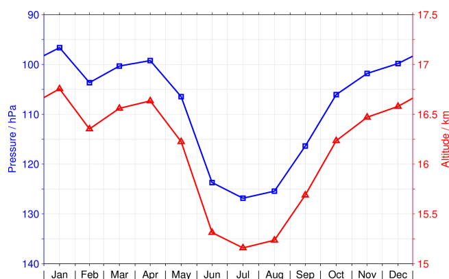
Figure 7. The annual variation of the start altitude for the HDO retrieval, i.e. the lowest altitude where sensible data can be derived from the MIPAS observations, considering data in the latitude range between 15^\circ S and 15^\circ N. The blue line shows the variation in pressure (uses the left axis), and the red line considers the geometric altitude (uses the right axis).
