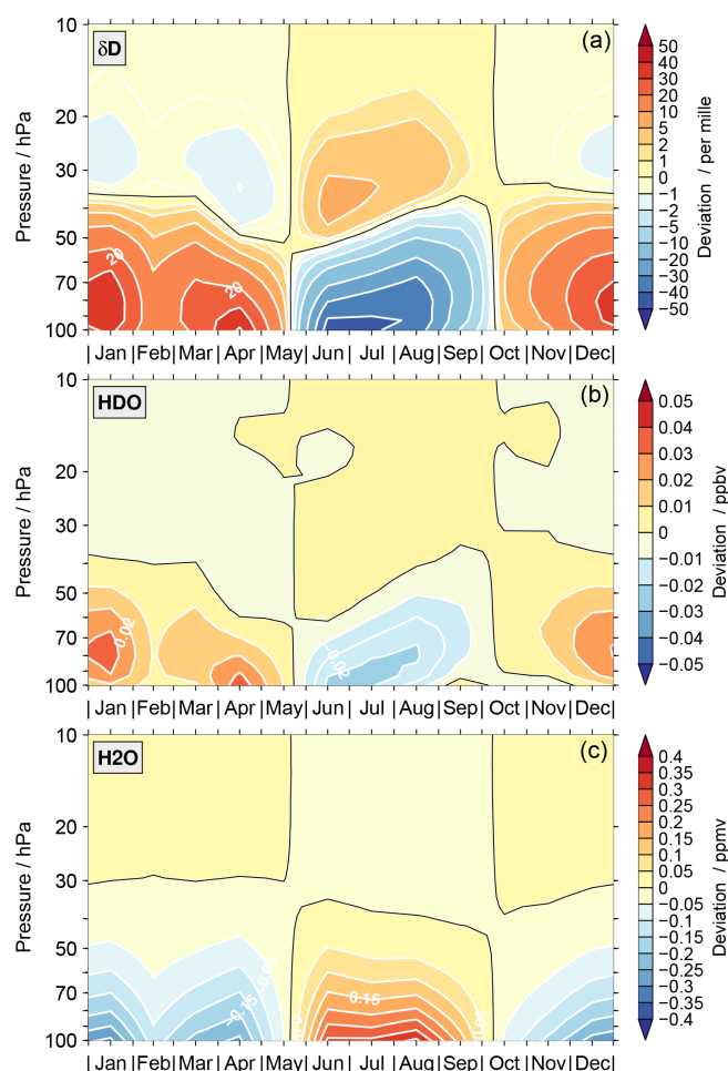
Figure 8. The approximated impact of the start altitude effect, in combination with temporal variation of the start altitude, on the annual variation of \delta D (a), HDO (b) and H_2O (c) calculated using Eq. (A15) in the Appendix.
