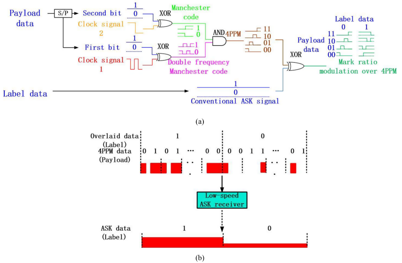
Fig. 2. (a) The generation reception of mark ratio modulation over 4PPM and (b) the reception for the overlaid mark ratio modulated signal (label signal).
