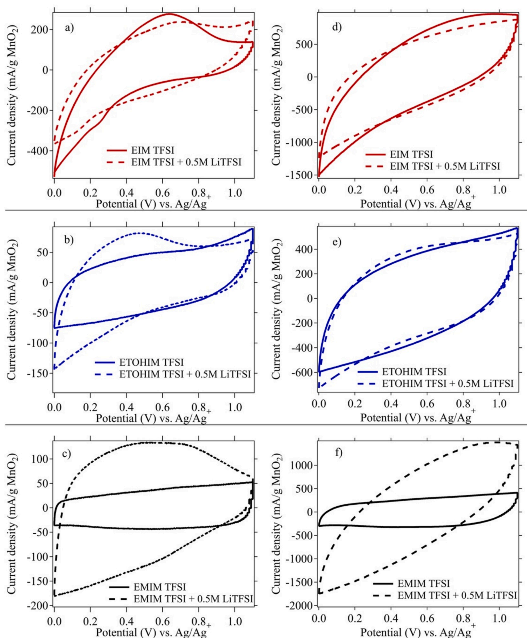
Fig. 5. Cyclic voltammograms of MnO 2 electrodes with a) EIM TFSI b) EtOHIM TFSI c) EMIM TFSI at 1 mV s -1 (left) and 20 mV s -1 (right) with and without the addition of 0.5 M LiTFSI.
