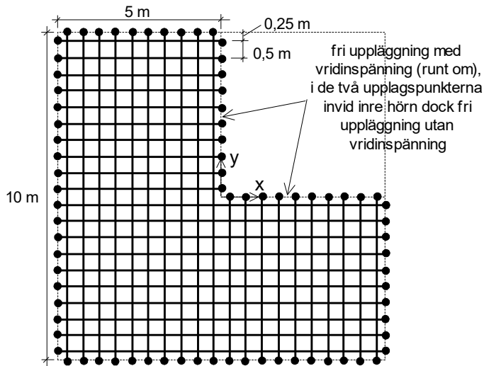
Figur C.4.1 Balkrostmodell.
