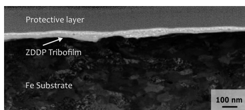
Figure 2 STEM image showing the cross-section of the tribofilm in the wear track. From top to bottom are Pt protective layer, ZDDP tribofilm and Fe substrate
