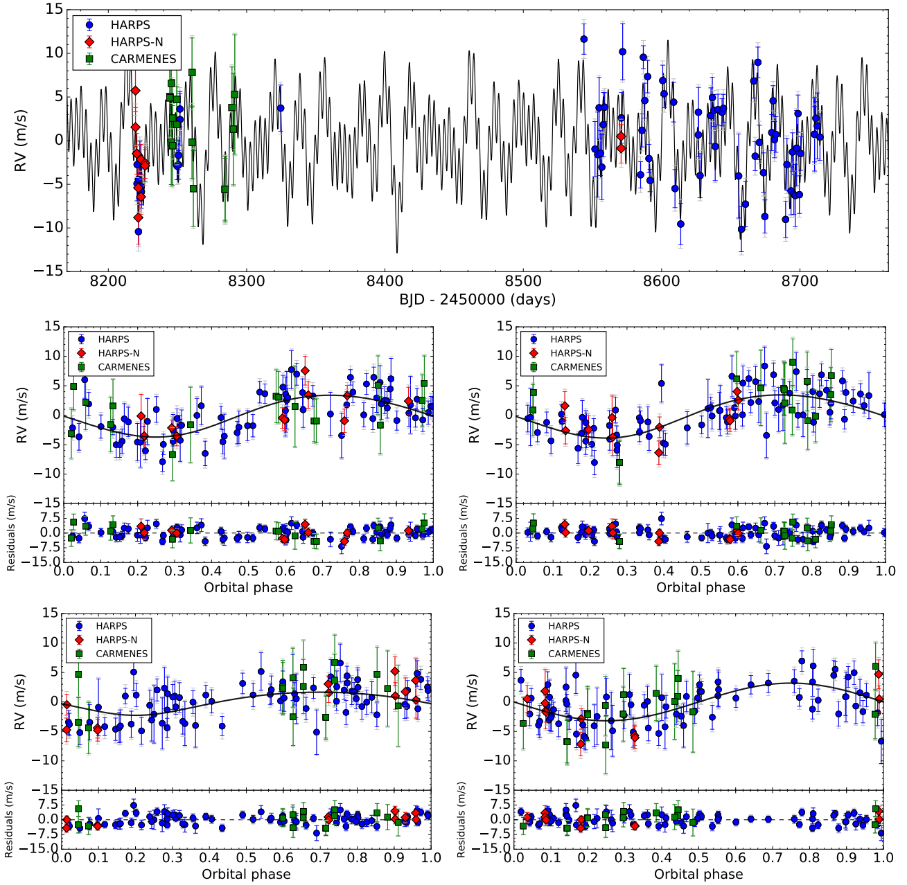
Fig. 7. Top panel: time series of the RV measurements of EPIC 249893012. Blue dots correspond to HARPS, red dots to HARPS-N, and green dots to CARMENES measurements. The best-fit model to the data is shown with a black thick line. The model includes three Keplerian curves and one sine curve mimicking the stellar signal at half the rotation period. Middle left panel: phase-folded RV measurements over the period of planet b after removing the signals from planets c and d and stellar activity. Middle right panel: phase-folded RV measurements over the period of planet c, after removing the signal from the other planets and stellar activity. Bottom left panel: phase-folded RV measurements over the period of planet d, after subtracting the signal from planets b and c and stellar activity. Bottom right panel: phase-folded RV measurements over half the rotation period of the star after removing the signals from the three planets.
