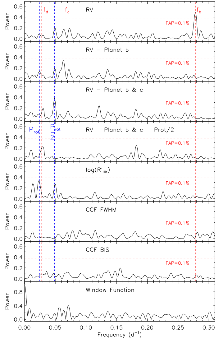
Fig. 6. Generalized Lomb-Scargle periodogram of the 2019 HARPS measurements ( upper panel ) and RV residuals, following the subtraction of the Doppler signals of planet b ( second panel ), planets b and c ( third panel ), and planets b and c plus the 20.5 d signal ( fourth panel ). The periodogram of the Ca II H & K lines activity indicator \log R'_{\text{HK}} , of the CCF BIS and FWHM, and of the window function are shown in the last four panels. The horizontal dashed lines mark the 0.1% FAP. The orbital frequencies of planets b, c, and d, as well as the stellar rotation frequency and its first harmonic are marked with vertical dashed lines.
