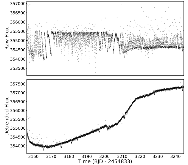
Fig. 2. K2 light curves of EPIC 249893012. Upper panel: raw light curve as extracted from the pixel data file in units of electrons per cadence. Lower panel: detrended light curve as obtained using our Everest-based pipeline. No stellar variability is detectable but the transit signals are clearly visible.
