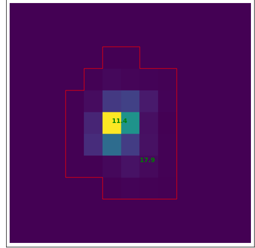
Fig. 1. Customized K2 image of EPIC 249893012. North is to the left and east at the bottom. The field of view is 43.78 \times 51.74 arcsec ( 3.98 arcsec per pixel). The red line marks the customized aperture for light-curve extraction, with a threshold of 1.7\sigma above the background. Green annotations are the Kepler magnitude (retrieved from the RA and Dec from MAST) of EPIC 249893012, and the source of contamination is identified in Fig. 5.
