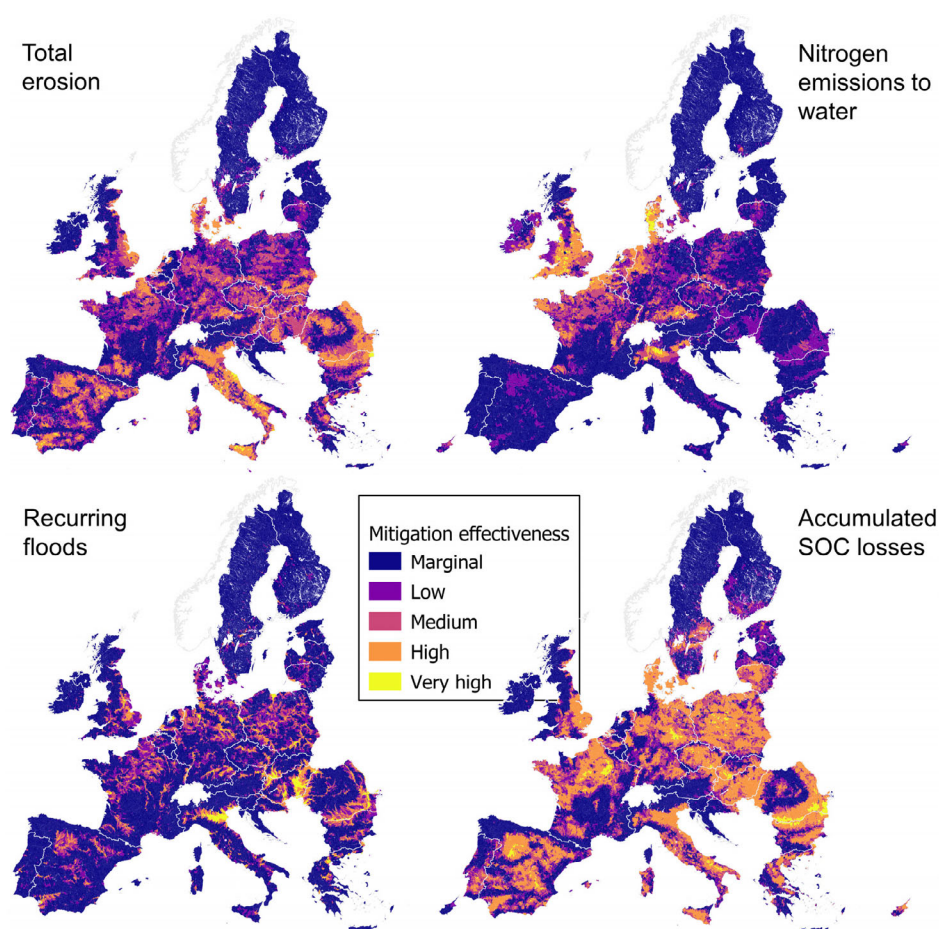
FIGURE 7 Estimated effectiveness of mitigating selected environmental impacts caused by intensive cultivation of annual crops, by a strategic introduction of perennials into the landscape (Englund et al., 2019)
